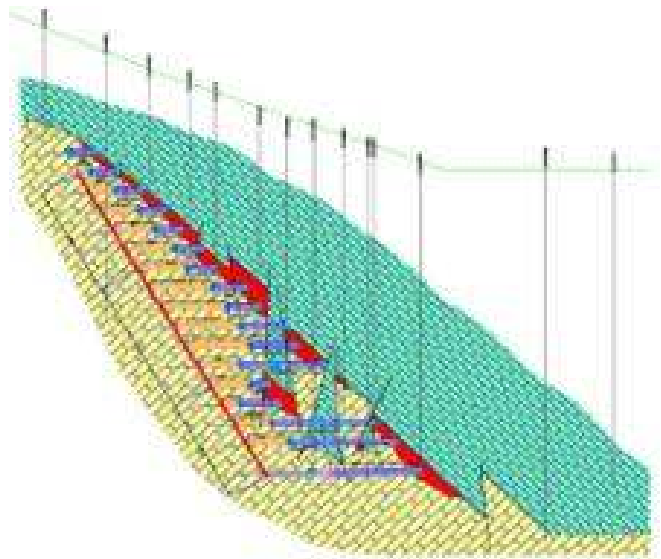
Mining works typical cross section
